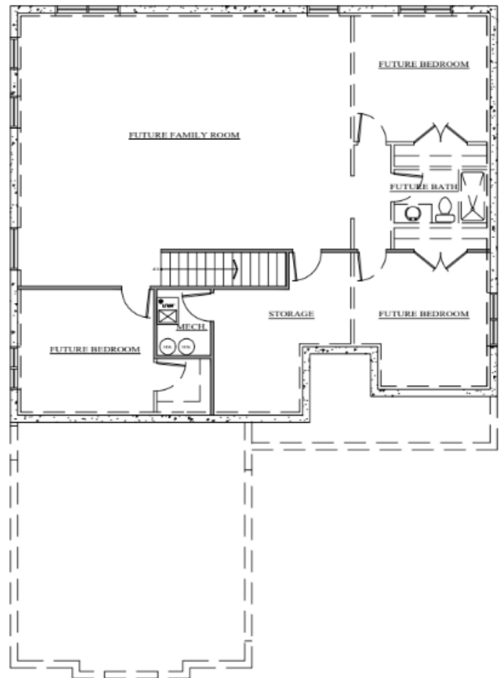
BASEMENT LEVEL (UNFINISHED)
