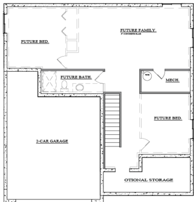
BASEMENT LEVEL (UNFINISHED)
