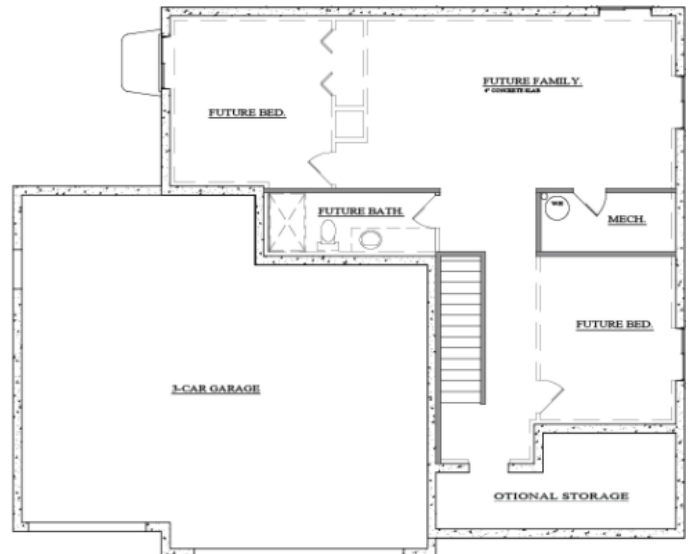
BASEMENT LEVEL (UNFINISHED)
