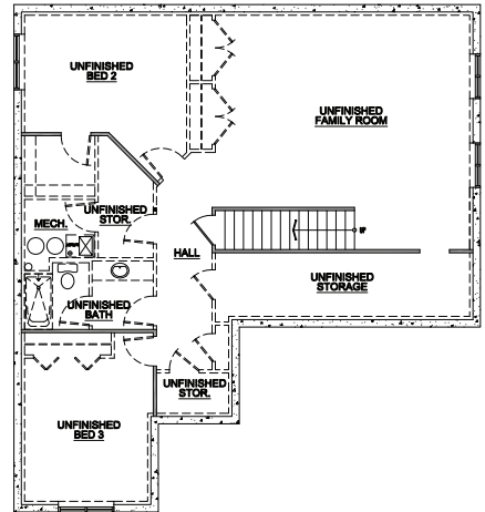
Lower Floor
